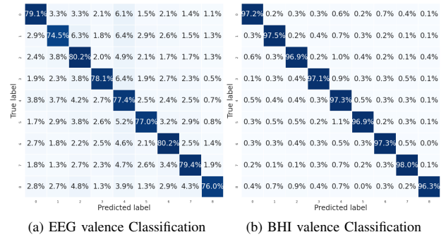
Fig. 2: Precision Confusion Matrices. Valence classification.
